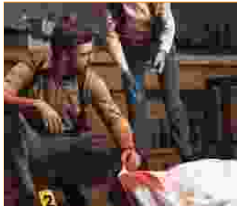
CSI Challenge
